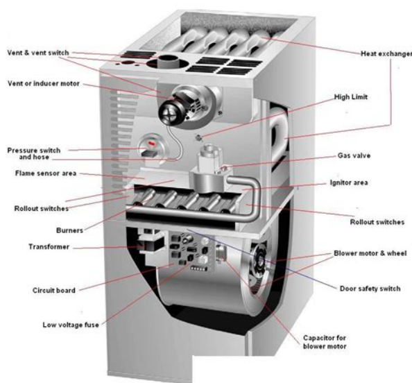
Typical component arrangement for a gas fired furnace.
